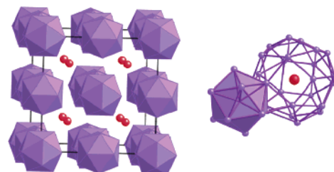
Figure 1. Crystal structure of CeBe 13 consists of Be 12 icosahedra (shown by purple shading) in a CsCl arrangement with Ce snub cubes. An isolated Be1 atom is located at the center of the Be 12 icosahedron, which is composed of Be 2 atoms. Red and purple circles represent Ce and Be atoms, respectively.
